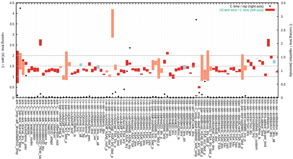
OCaml (4.07.0) native code performance over C (cc -O3 -Wall -Werror -fPIC), 99.5% confidence
